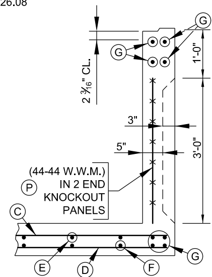
SECTION 2-2
